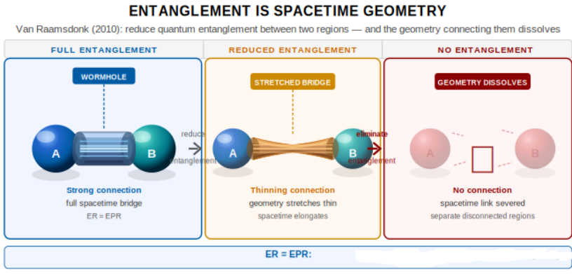
Figure 15 - 1 2Van Raamsdonk (2010): "Building up spacetime with quantum entanglement." The degree of entanglement between boundary regions corresponds precisely to geometric connectivity in the bulk spacetime.
